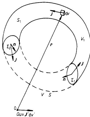
Figure 1. The geometry of the current distribution \mathbf{J} and the volume current element \mathbf{J}' d\mathbf{v}' at the origin.
